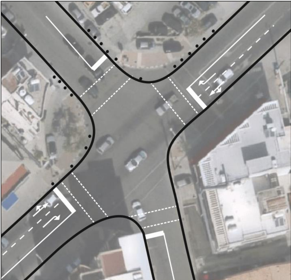
Figure A-VII 7: Accident Accumulation Zone 4: position of poles on sidewalks
